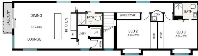
SECOND FLOOR
